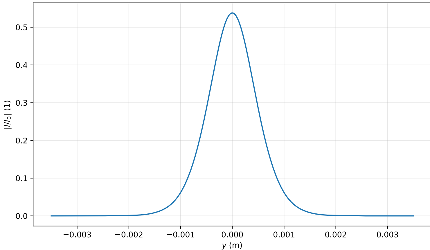
Intensity profile I(x=0, y, z=3.662)/I_0 , P_{in}=0.6P_{cr} , artificial time
